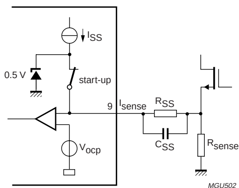
Fig.10 Soft start.
